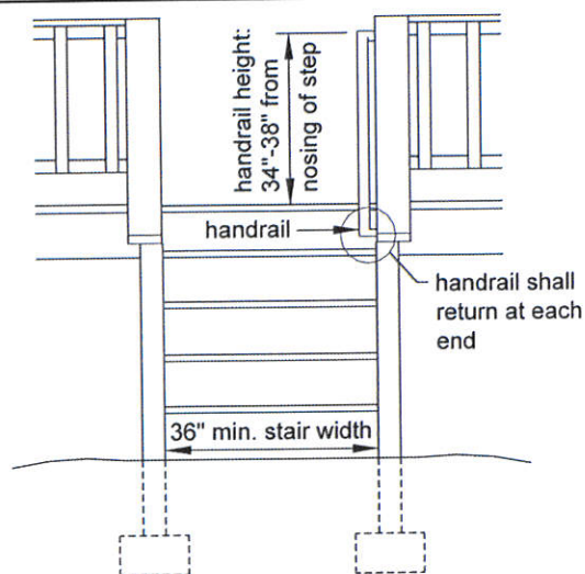
Figure 33. Miscellaneous Stair Requirements.
