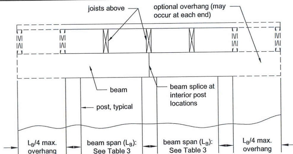
Figure 3. Beam Span.
